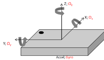
Figure 9 BHA, BHI and BMG250 axes orientation
