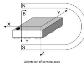
Figure 5 BMM155 axes orientation in datasheet
